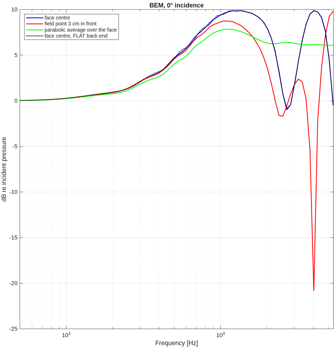
BEM, 0°: centre, field point 3 cm in front, parabolic average over the face, and flat back end.
